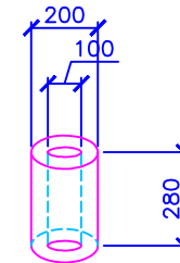
DETAILS OF CYLINDRICAL RUBBER FENDER (SIZE:- 200 mm O.D X 100 mm ID X 280 mm LONG)
