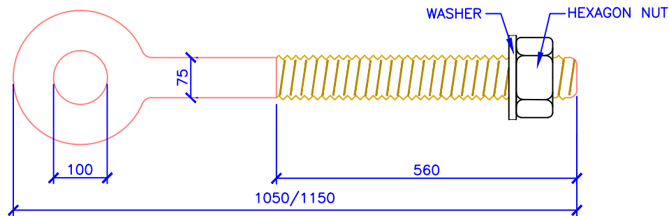
DETAILS 75 mm EYE BOLT
