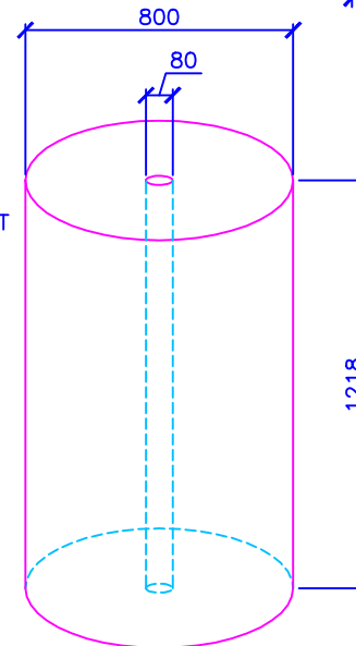
DETAILS OF CYLINDRICAL RUBBER FENDER (SIZE:- 800 mm O.D X 80 mm ID X 1218 mm LONG)
