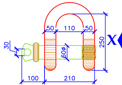
DETAILS 50 mm DEESHACKLE
