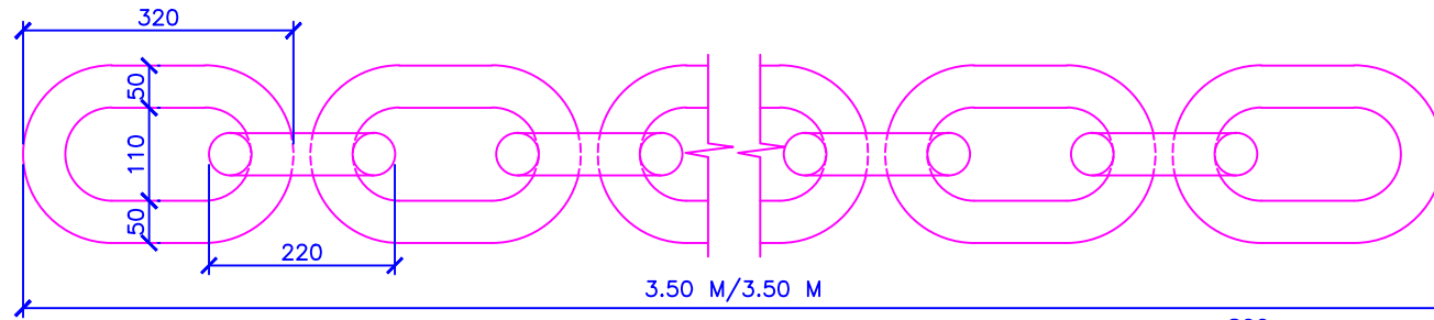
DETAILS 50 mm Ø CHAIN
