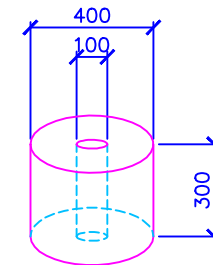
DETAILS OF CYLINDRICAL RUBBER FENDER (SIZE:- 400 mm O.D X 100 mm ID X 300 mm LONG)
