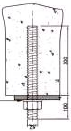
DETAILS OF RESIN ANCHOR BOLT ASSEMBLY
