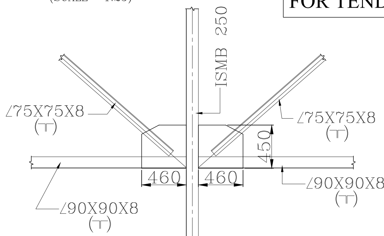
DETAIL: X (SCALE- 1:25)
