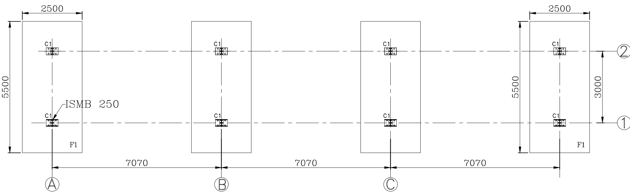
LAYOUT PLAN OF COLUMN FOUNDATION (SCALE- 1:100)
