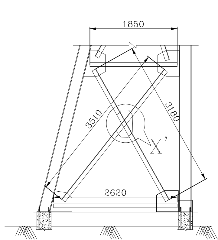
SIDE ELEVATION (SCALE- 1:100)
