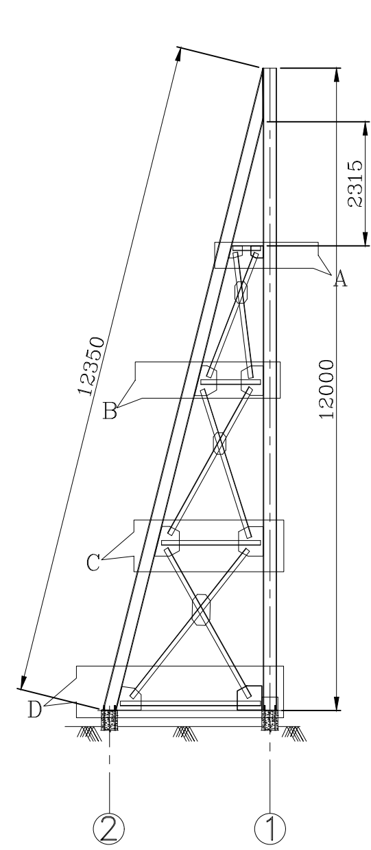
MEMBER DIMENSION (SCALE- 1:100)
