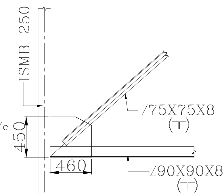
DETAIL: X (SCALE- 1:25)
