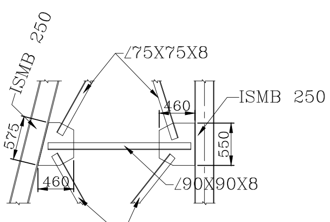
DETAIL-C (SCALE- 1:50)
