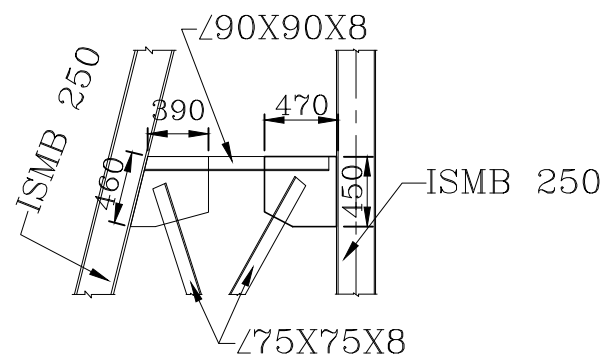
DETAIL-B (SCALE- 1:50)
