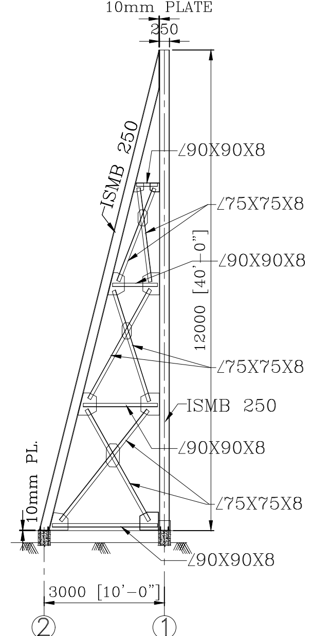
SIDE ELEVATION (SCALE- 1:100)
