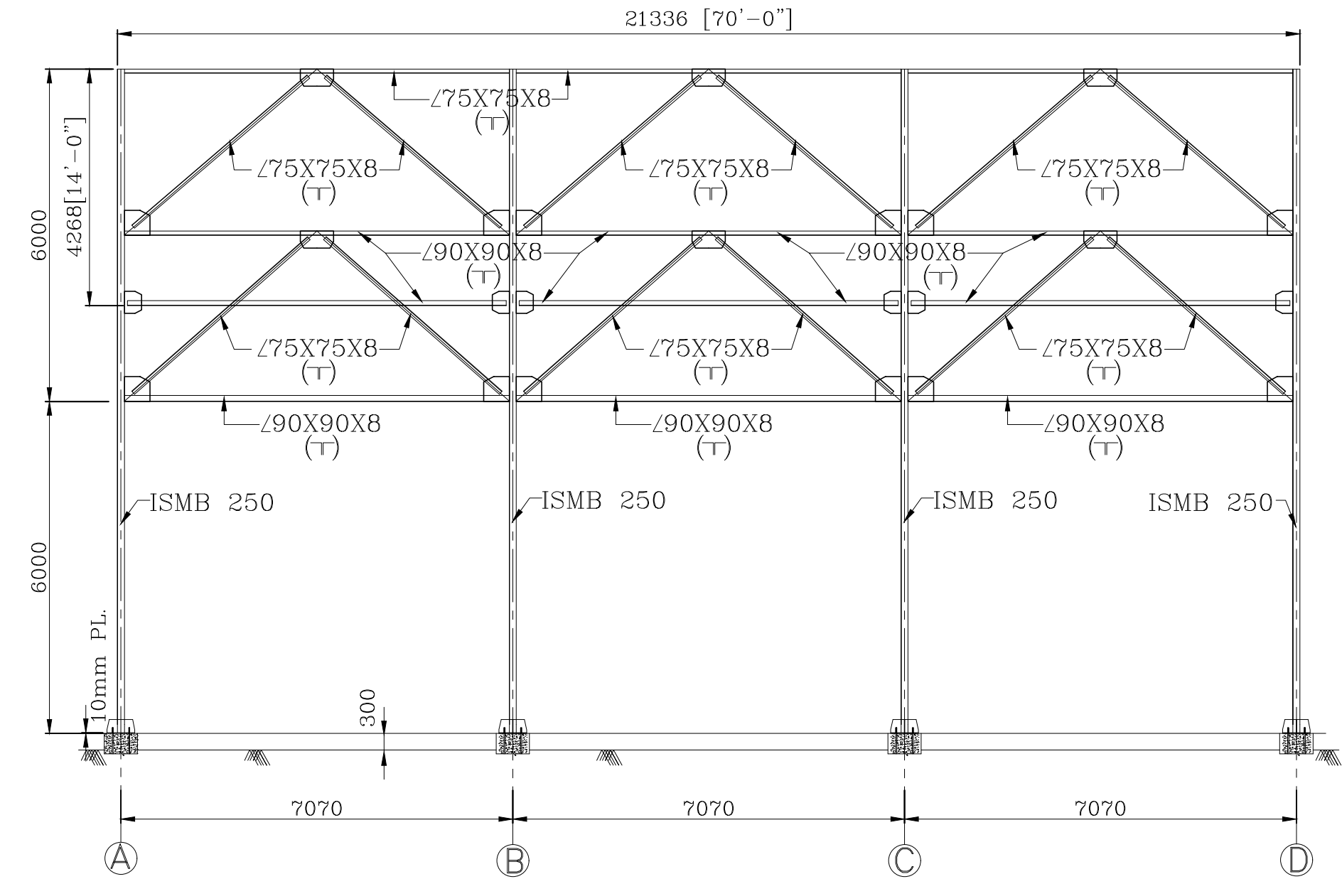
ELEVATION (SCALE- 1:100)
