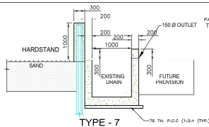
TYPE - 7 (DRAIN MODIFICATION + RETAINING WALL)
