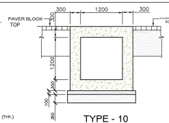
TYPE - 10 (UNDER GROUND DRAIN)
