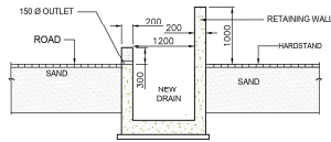
TYPE - 2 (NEW DRAIN WITH RETAINING WALL)
