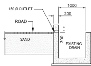
TYPE - 1 (DRAIN MODIFICATION)
