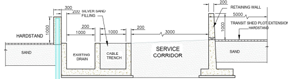
TYPE - 5 (RETAINING WALL ON EXISTING DRAIN + CABLE TRENCH WITH RETAINING WALL + SERVICE CORRIDOR 3 MTRS)
