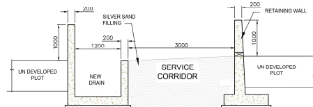
TYPE - 9 (NEW DRAIN WITH RETAINING WALL + SERVICE CORRIDOR)
