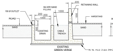
TYPE - 3 (DRAIN MODIFICATION + CABLE TRENCH WITH RETAINING WALL)
