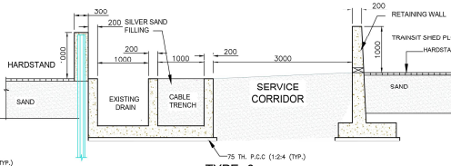
TYPE - 6 (RETAINING WALL ON EXISTING DRAIN + CABLE TRENCH WITH RETAINING WALL + SERVICE CORRIDOR 3 MTRS)
