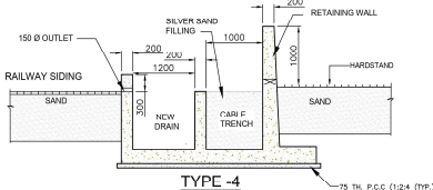
TYPE - 4 (NEW DRAIN + CABLE TRENCH WITH RETAINING WALL)
