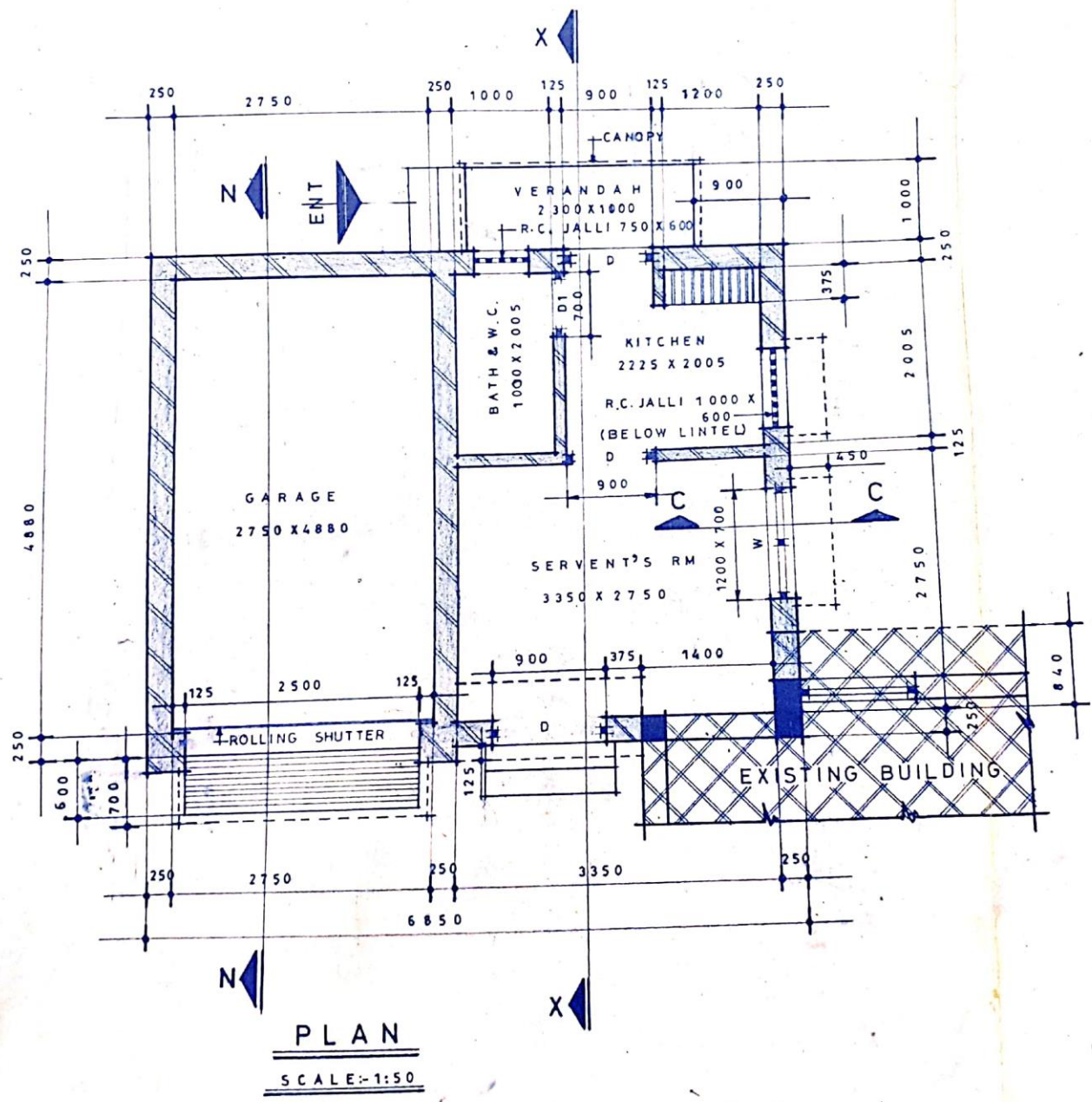
Figure 1: Plan: Garage & Servants Quarter
