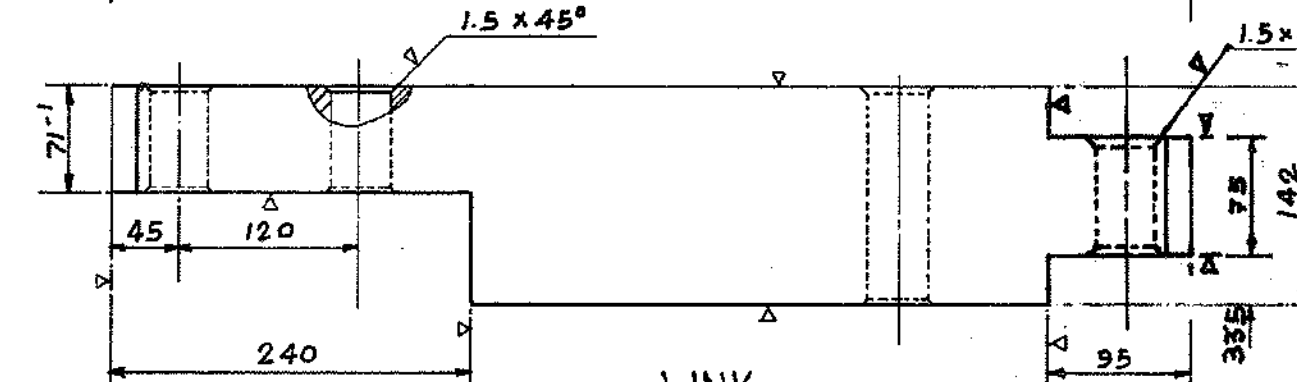
LINK WEIGHT-67.66 KG. (approx.) DRG. NO. 210-085/3 REF. BC1/04.00.00.04A 1. HOLES MARKED BY ▼ SHOULD BE DRILLED IN ASSEMBLY.
