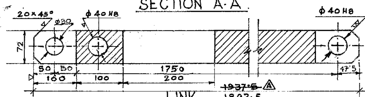
LINK WEIGHT - 152.5 KG. (approx.) DRG. NO. 210-085/4
