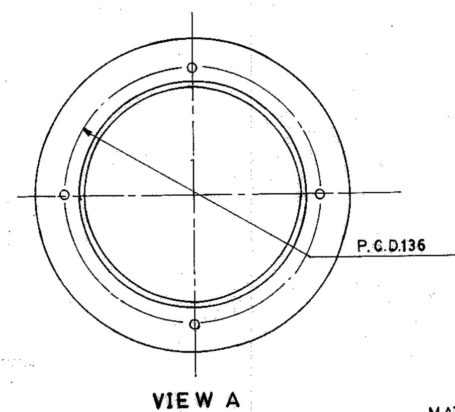
VIEW A
