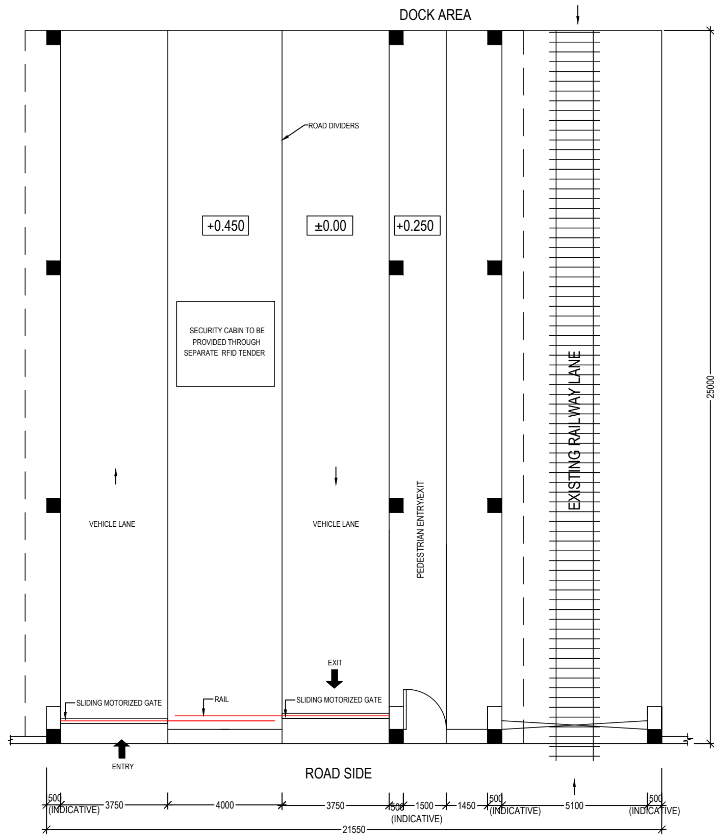
PLAN AT GATE NO.4
