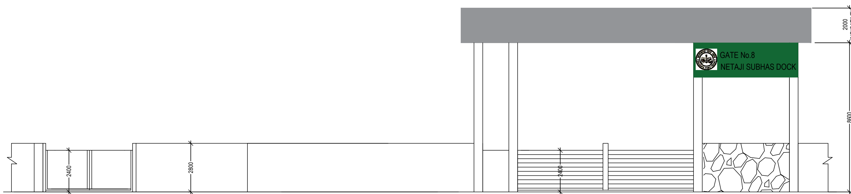
ELEVATION AT GATE NO.8
