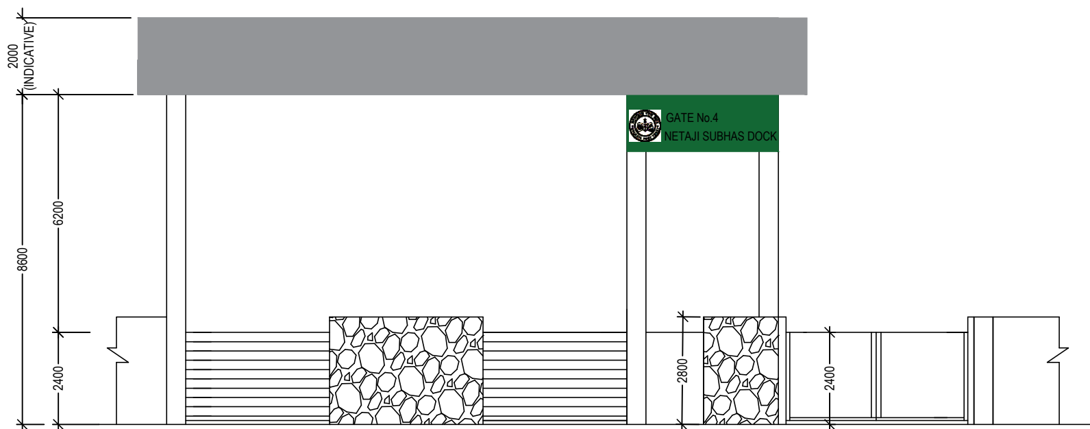
ELEVATION AT GATE NO.4
