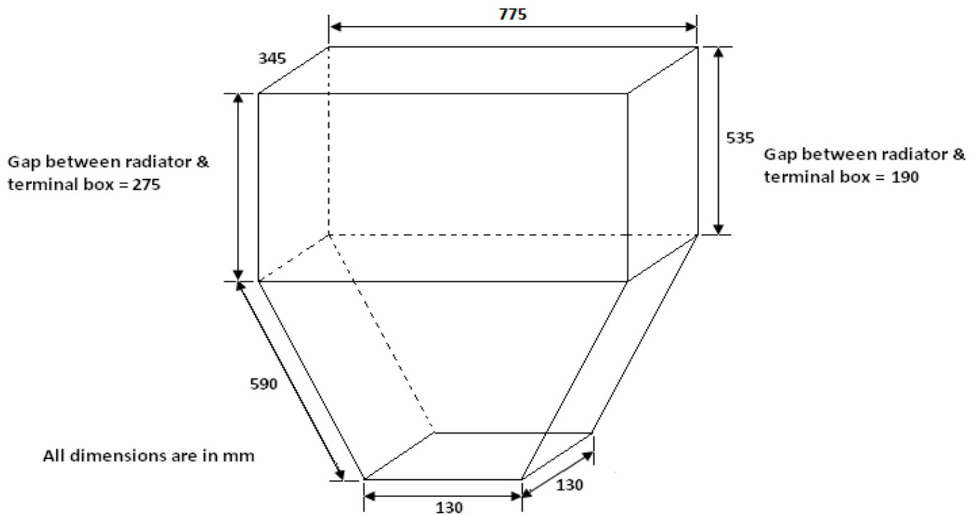
HV Terminal Box of 6 MVA 33 KV / 3.3 Transformer of Master Control Sub-Station
